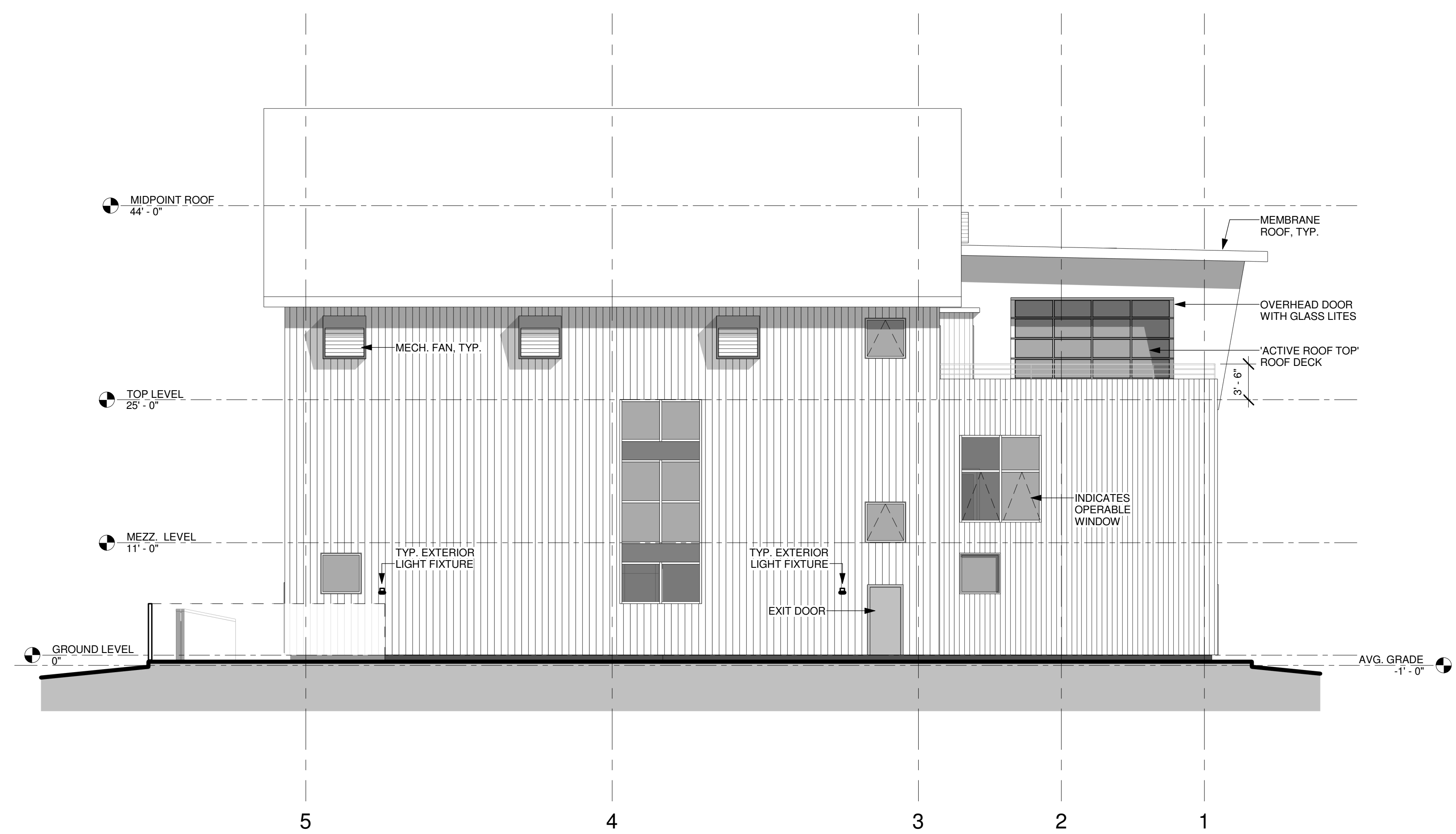
1 WEST FACING ELEVATION 1/8" = 1'-0"
