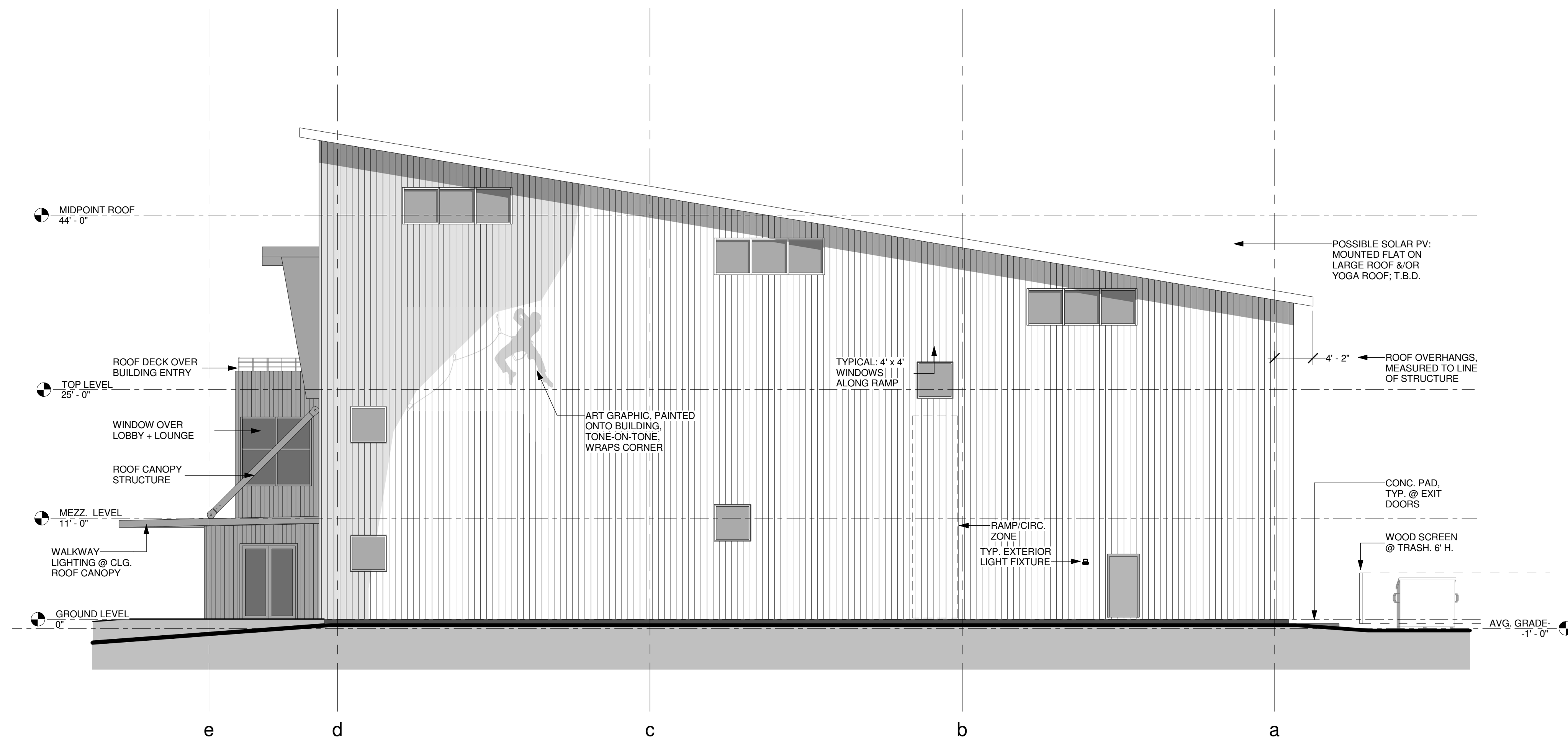
1 NORTH FACING ELEVATION 1/8" = 1'-0"
