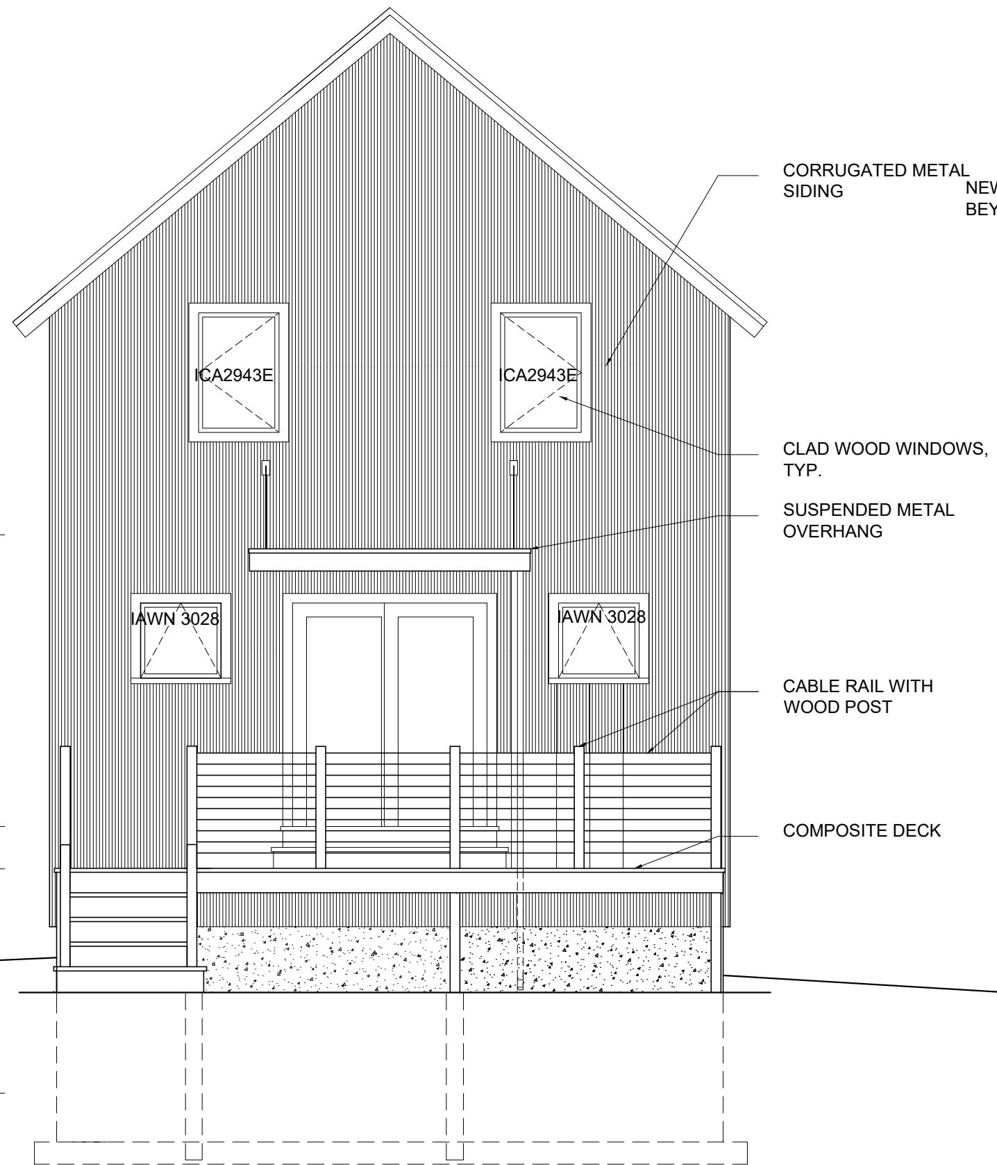
1 PROPOSED NORTH ELEVATION
